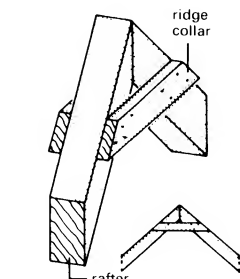
12 Ridge collar connecting two rafters
